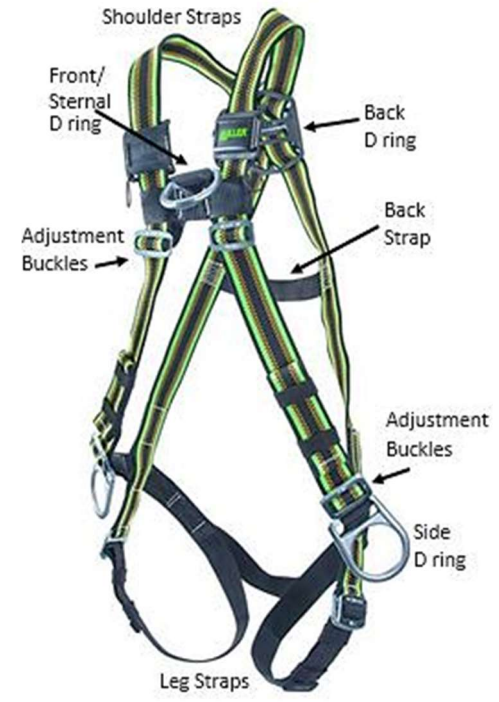
Fall Protection Harness
