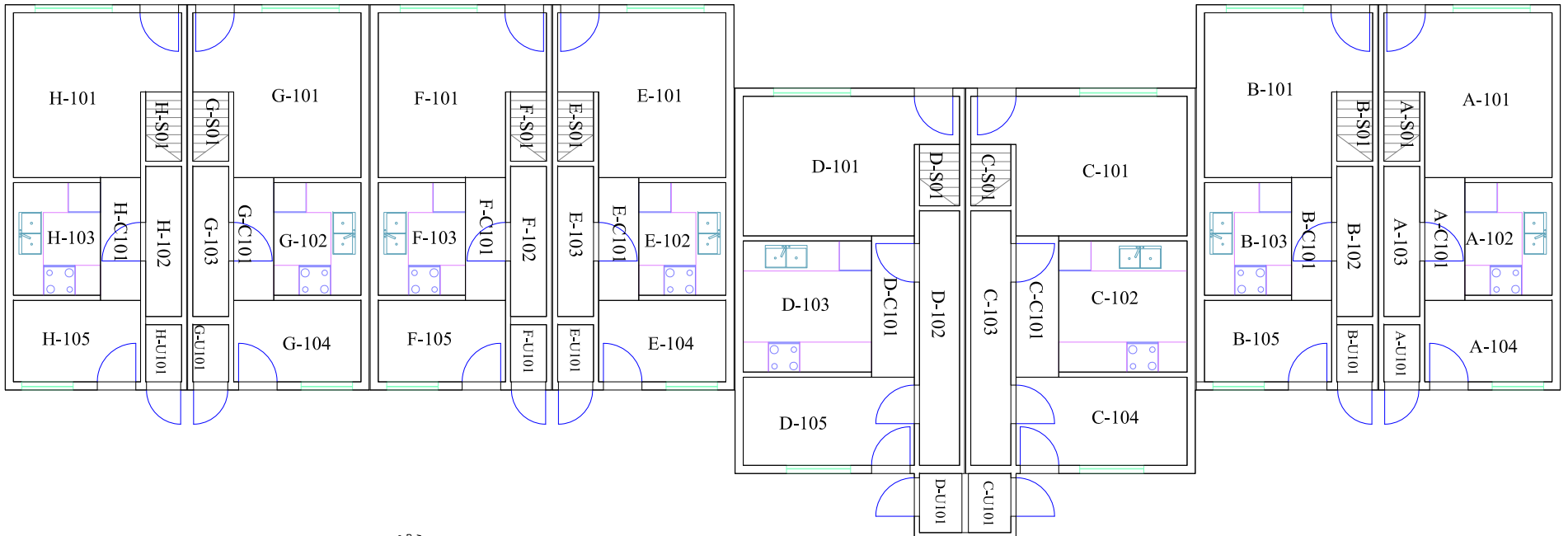
FIRST FLOOR TOWNHOUSE APTS. BUILDING 4
