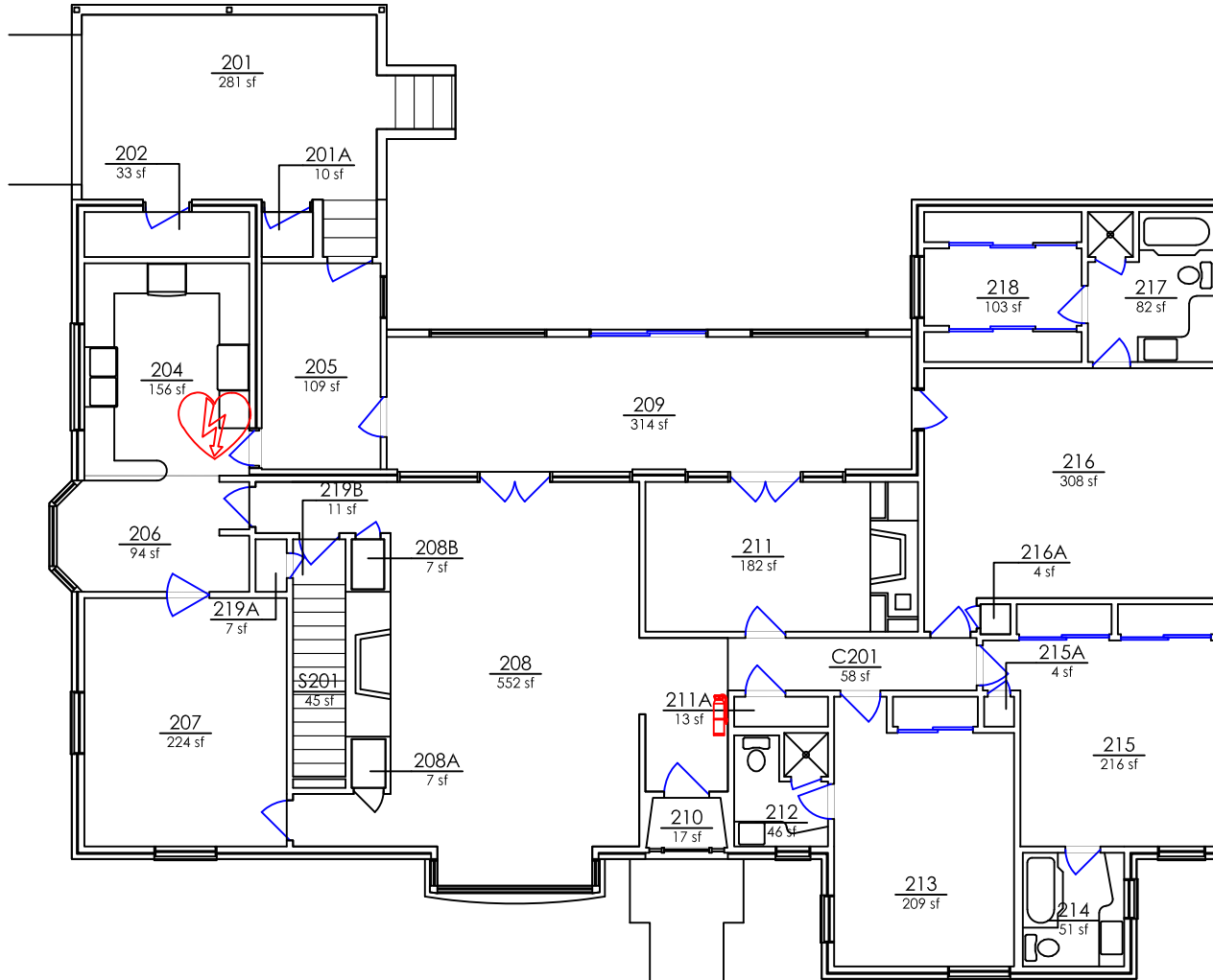
FIRST FLOOR GOVERNOR MARTIN HOUSE
