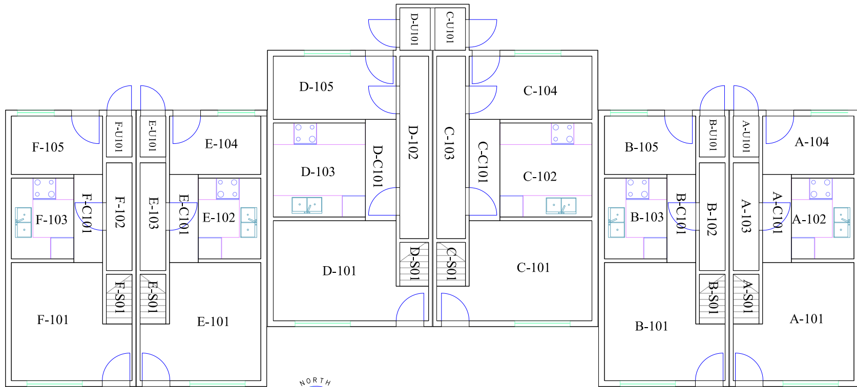
FIRST FLOOR TOWNHOUSE APTS. BUILDING 10
