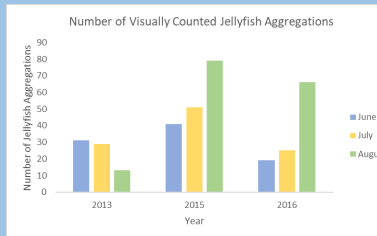
Figure 2: The above bar graph depicts a similar comparison between the same three years. Even without the image analysis process providing area data, an increase in the number of aggregations from 2013 to 2016 is apparent.
