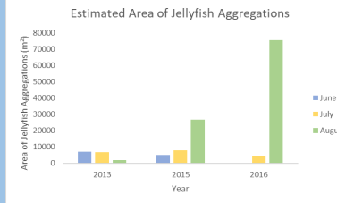
Figure 1: The above graph shows a comparison between three separate years. A pattern of increasing estimated area of jellyfish aggregations can be observed, especially in the month of August when the jellyfish tend to bloom. This data could suggest that the unusually high temperatures in 2015 and 2016 had a positive effect in jellyfish abundance.
